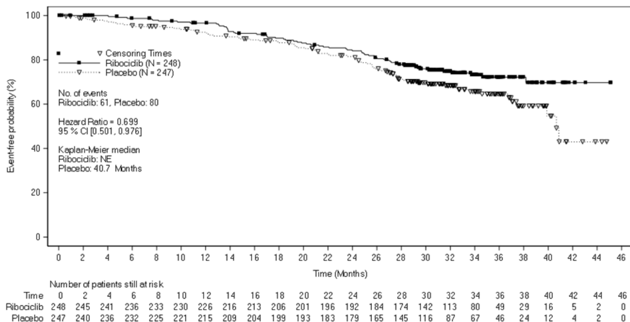
Figure 5 MONALEESA-7: Kaplan Meier plot of final OS analysis in patients who received NSAI (30-Nov-18 cut-off)
