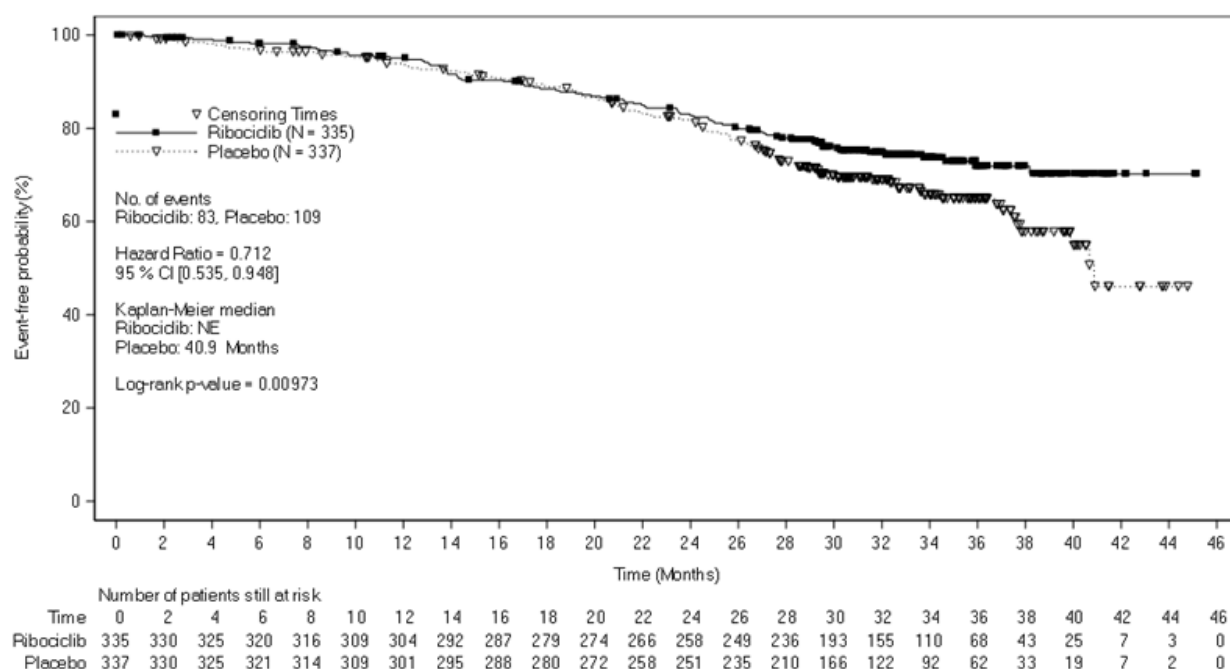
Figure 4 MONALEESA-7: Kaplan Meier plot of final OS analysis (30-Nov-2018 cut-off)
