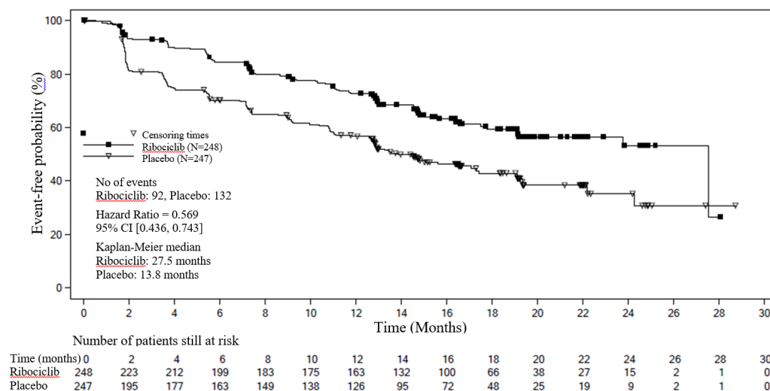
Figure 3 MONALEESA-7 – Kaplan-Meier plot of PFS based on investigator assessment in patients who received NSAID
