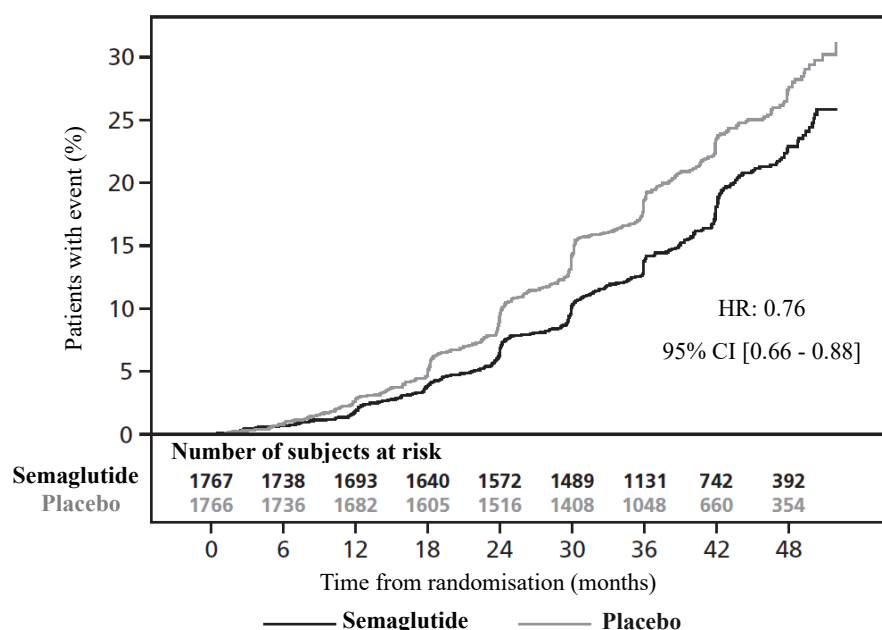
Figure 9: Cumulative incidence function of time to first occurrence of the primary composite outcome: onset of persistent \geq 50\% reduction in eGFR, onset of persistent eGFR < 15 \text{ mL/min/1.73 m}^2 , initiation of chronic kidney replacement therapy, kidney death or cardiovascular death (FLOW)
